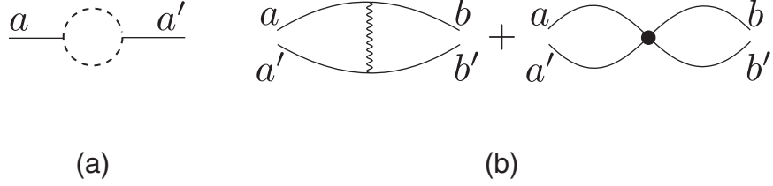
Figure 6.2 Possible quantum corrections to scalar propagators in \mathcal{N} = 4 Super Yang–Mills theory at order g_{\text{YM}}^2 . (a) Self-energy correction from a fermion loop. (b) Exchange contributions: gauge boson exchange and quartic scalar interaction.
